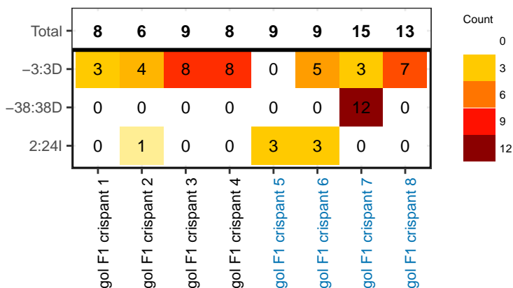
Figure 4: plotFreqHeatmap with X-axis labels coloured by experimental group and tiles coloured by count instead of proportion
