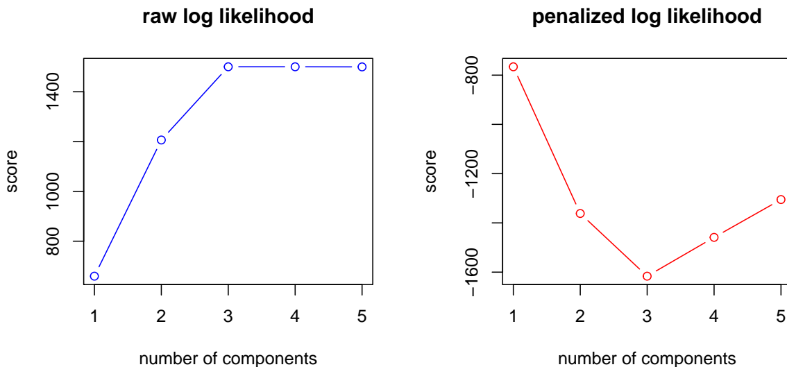
Figure 4: Model selection
