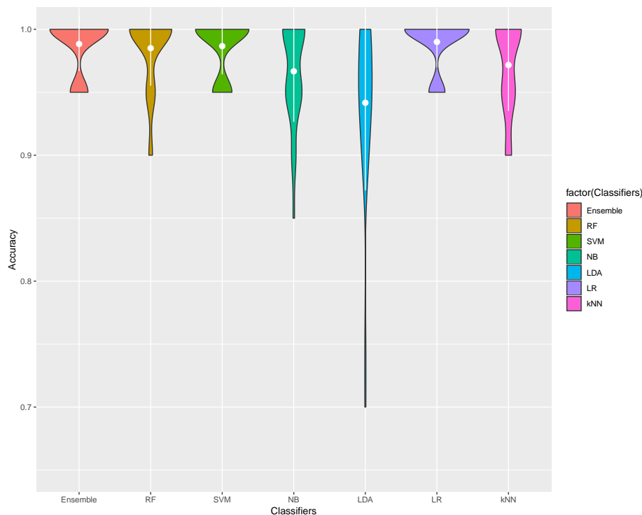
Figure 12: Accuracies Comparison The violin plot highlights the classification accuracy of each classifier, computed at each iteration; a black dot represents a specific accuracy value while the shape of each “violin” is drawn by a Gaussian kernel density estimation. Averaged accuracies and standard deviations are represented by white dots and lines.
