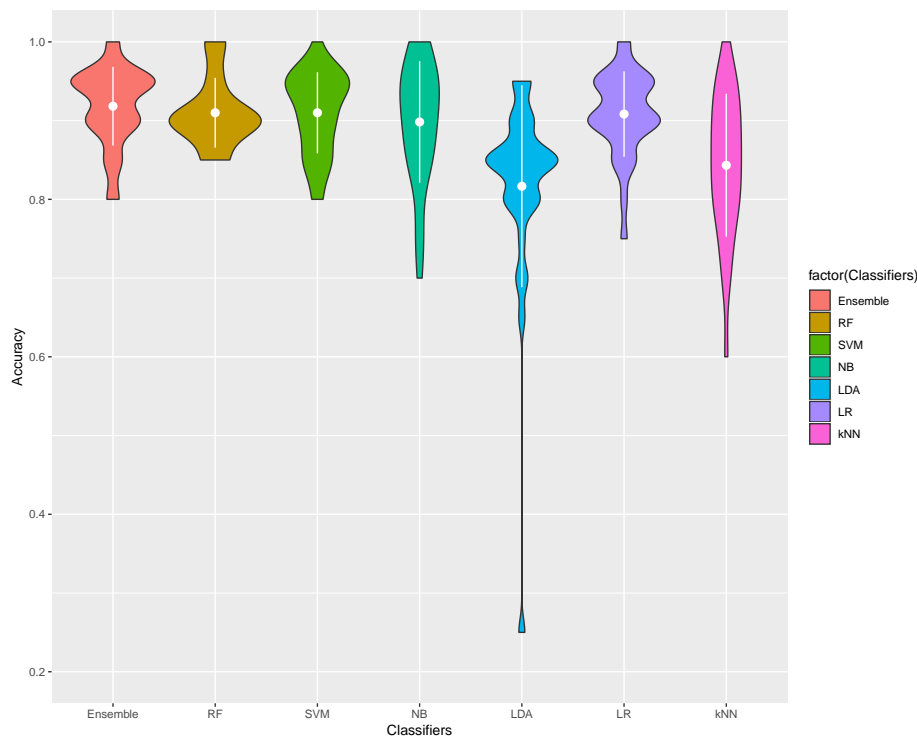
Figure 13: Accuracies Comparison
