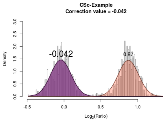
Figure 1: plotDensity
