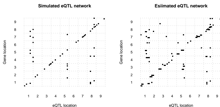
Figure 4: Dot plots of eQTL associations in a simulated eQTL network (left) and in an estimated eQTL network (right) selecting marginal associations at FDR < 5\% and non-rejection rate with \epsilon < 0.1
