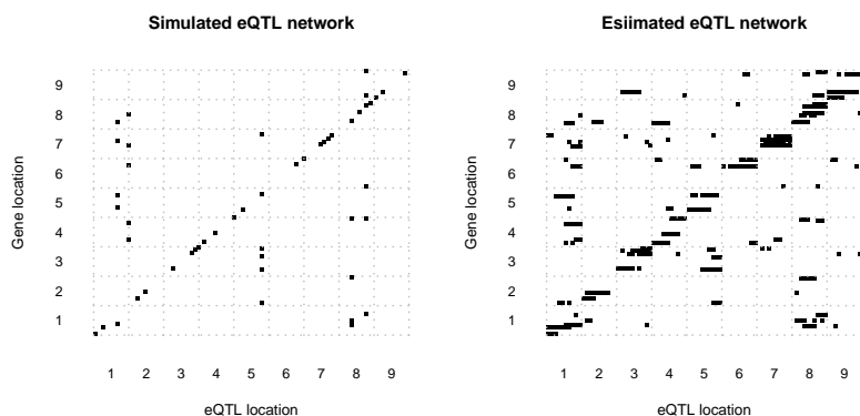
Figure 3: Dot plots of eQTL associations in a simulated eQTL network (left) and in an estimated eQTL network (right) selecting marginal associations at FDR < 5% and non-rejection rate meeting a cutoff \epsilon < 0.1
