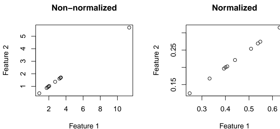
Figure 3: Non-normalized and normalized associations between feature 1 and feature 2
