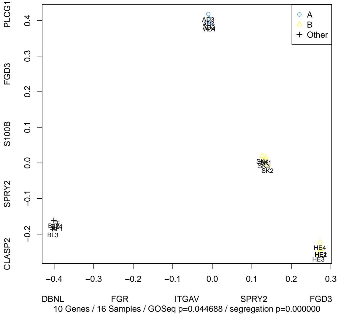
Figure 9: OUT\SCGO\Scatter.Ax4.Bx8.GO0001726.pdf The Scatter file is similar to the PCA files, but the gene set is restricted to those within a given, significant, GO Term. As in the PCA file, genes driving the principle components are annotated along the axes. At the bottom of the figure, statistics are given pertaining to this group. All such data is available in tables, but this Scatter plot helps the user see which samples behave like which groups. Depending on the number of genes relative to the number of samples, different PCA formulas may be used. For a set with only two genes, this file can directly display the expression values as normalized counts, the same as found on the expression heatmap (Fig. 6.)
