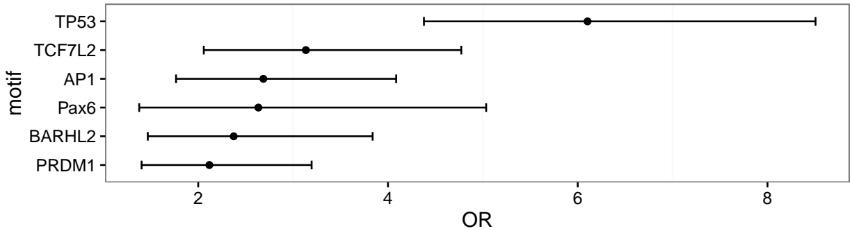
Figure 6: The plot shows the Odds Ratio (x axis) for the selected motifs with OR above 1.3 and lower boundary of OR above 1.3. The range shows the 95% confidence interval for each Odds Ratio.
