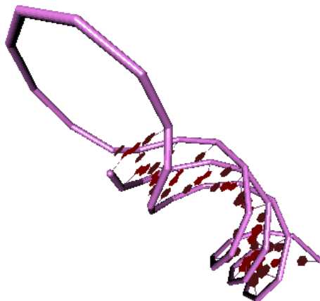
Figure 4: 3D scheme of detected triplex
