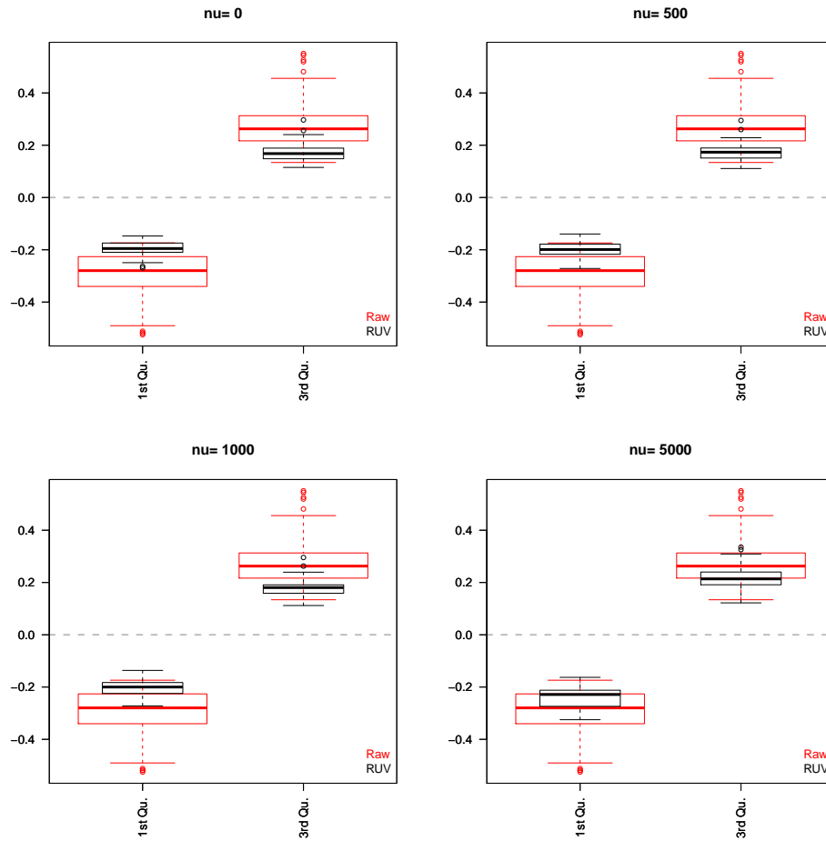
Figure 5: RLE plots comparing different options of \nu for \hat{k} = 3 The boxplots summarize the 25% and 75% quantile of all samples. The red boxplots display the raw data, while the black boxplots refer to the RUV applied with \hat{k} = 2 and \nu as in the title of the panel.
