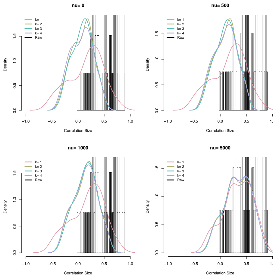
Figure 3: Impact of different parameter choices on the correlations of a set of sodium channel genes Correlation densities for different parameter choices. The histogram in the background of each panel shows the density of the correlations of the random genes calculated using the raw data.
