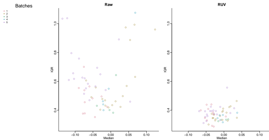
Figure 6: RLE plots for data cleaned with RUV using \nu = 500 for \hat{k} = 2 Every sample is represented by the median and inter-quantile-range of the difference between observed gene expressions and study mean. The samples are colored according to their batches.
