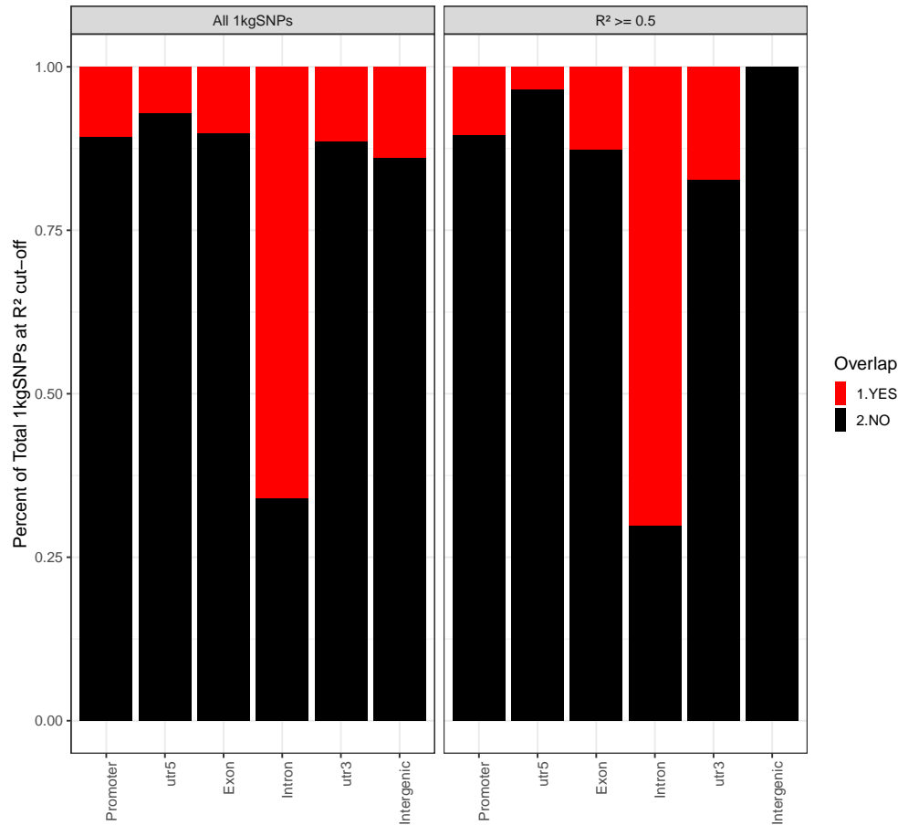
Distribution of 1kgSNP SNPs across Genomic Features at R^2 cut-off of 0.5
