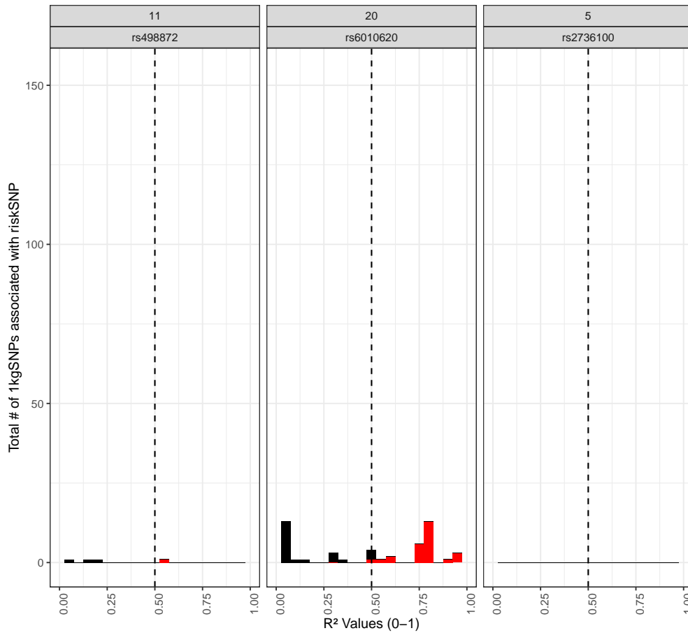
Figure 5: Histogram distribution of number of correlated SNPs at each Rsquare value
