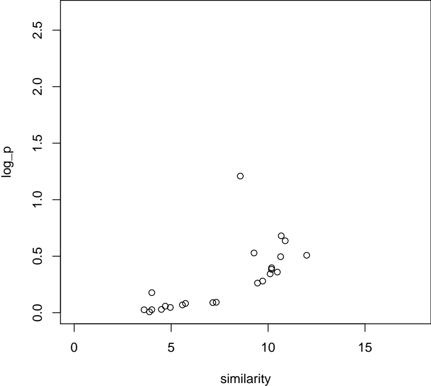
volcano plot
