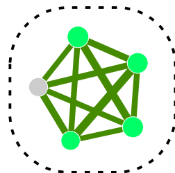
module12 (p.value=7.72e-03)
