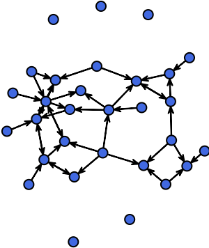
Priors weight = 0.25
