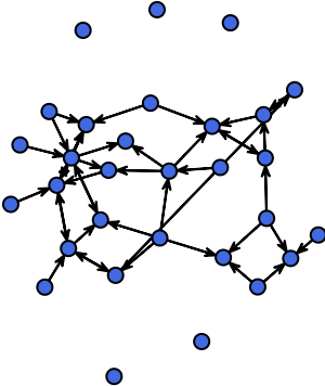
Priors weight = 0.75
