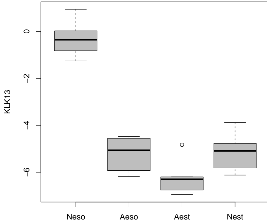
Boxplot for Tissue sample label
