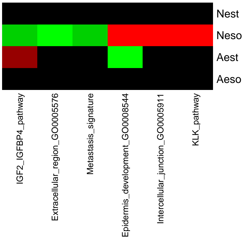
Figure 8: Result from functional classification of gene groups for “Tissue” label.
