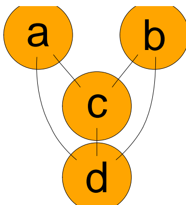
Figure 1: The graph g1 .
