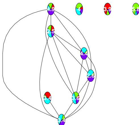
Figure 12: g1 with pie charts as nodes.
