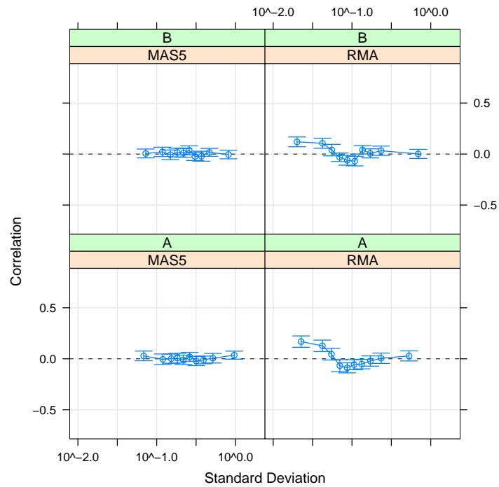
Figure 4: Multiple correlation plot, showing the correlation plot for MAS5 and RMA values for both dataset A and B.
